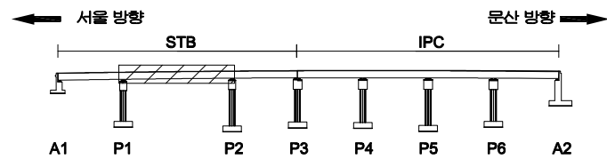
KEY PLAN
